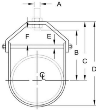
CB-235 Standard Clevis Hanger Dimensions
