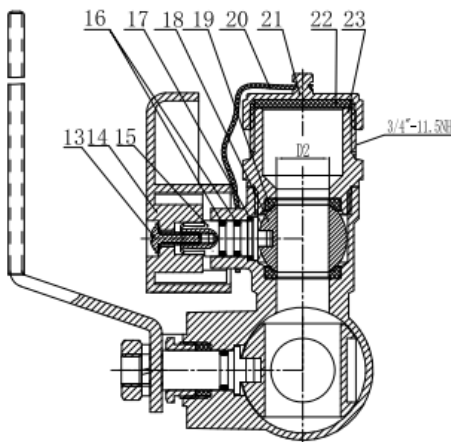
A-A Section view
